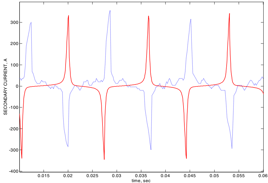
Fig.36. Case 3 – secondary currents: test (dotted blue) and simulation (red). The currents are inverted for better visualization. A 32kA test of the C5 CT.
