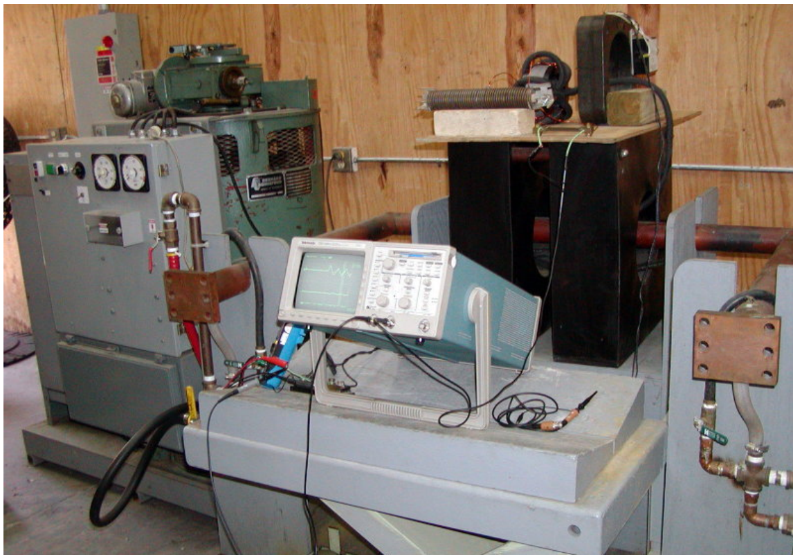
Fig.31. Test setup.
