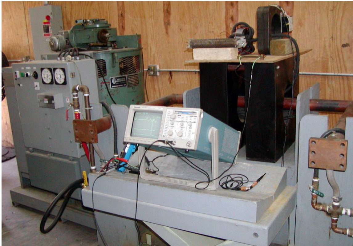
Fig.31. Test setup.
