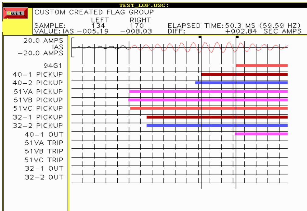
Figure 4 Typical Digital Flags captured by a digital protection system. (File: test_lof.bmp)
