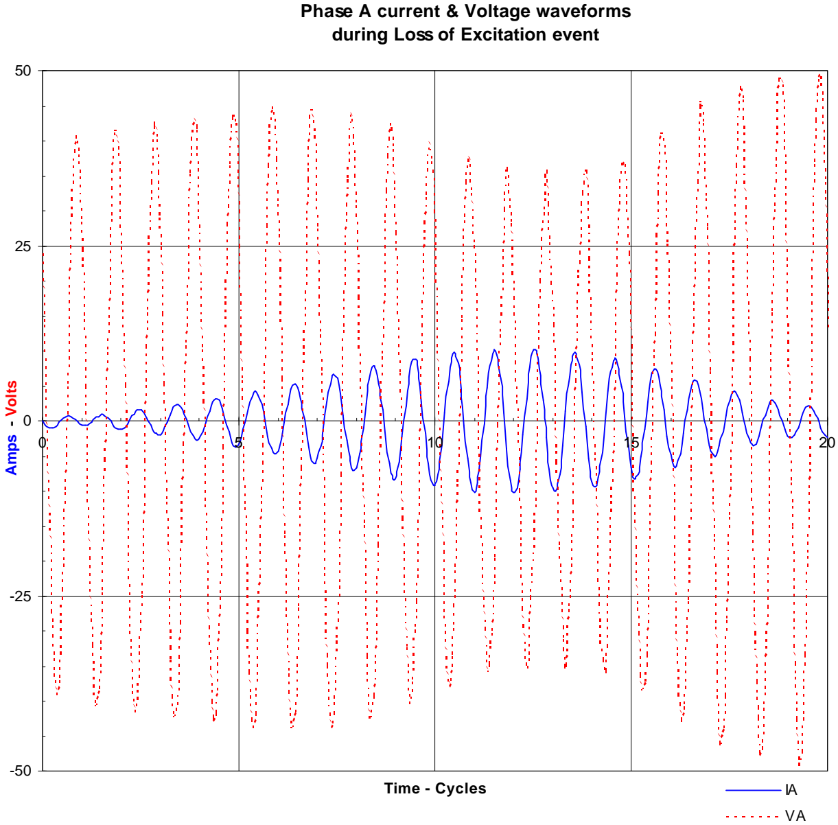
Figure 3 Typical waveforms captured by a digital protection system. (File: test_lof.xls)
