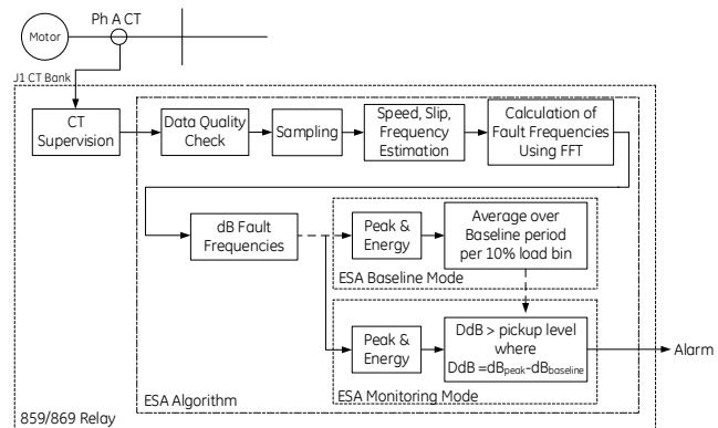
Figure 1: 859/869 ESA Architecture
