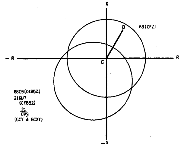
R-X CHARACTERISTIC OF CARRIER STARTING UNITS
