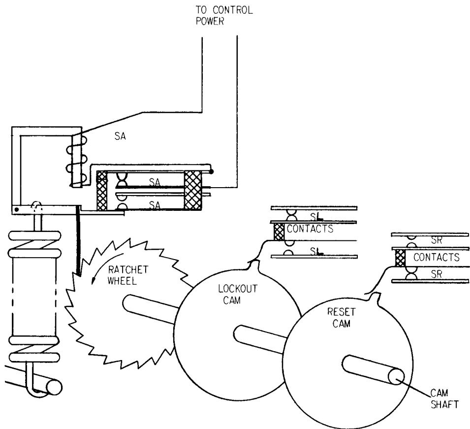
Fig. 2. Stepping switch for NLR relay (0178A9144)
