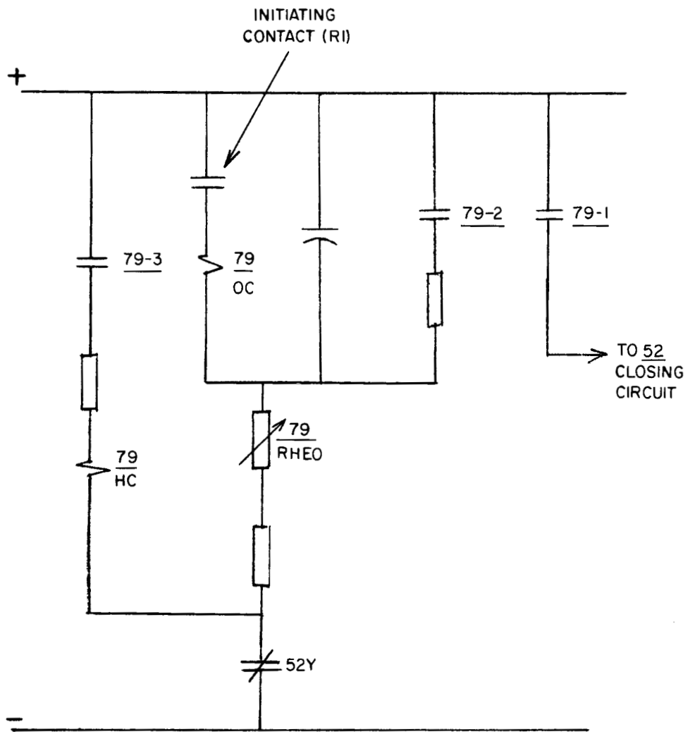
Fig. 12. Simplified diagram of NSR reclosing relay circuit
