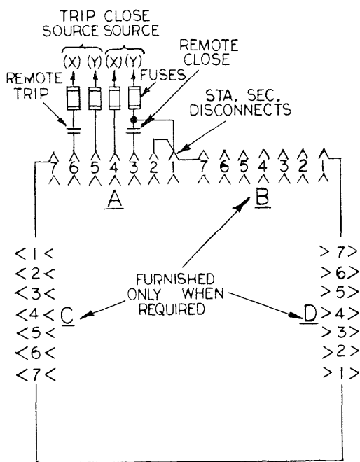
FRONT VIEW AK-1A-15, 25 & AK-2A-15, 25 BREAKER COMPARTMENT
