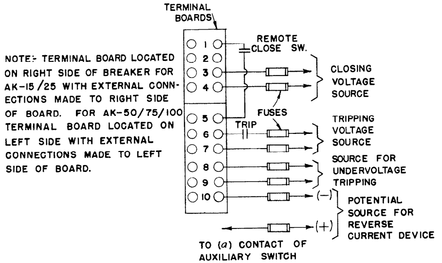
Fig. 1 (Front View)
