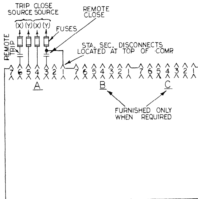
FRONT VIEW AK-2A-50, 75, 100 BREAKER COMPARTMENT
