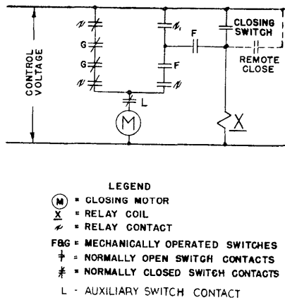
Fig. 7 Simplified Elementary Diagram Internal Wiring AK-50, 75 and 100
