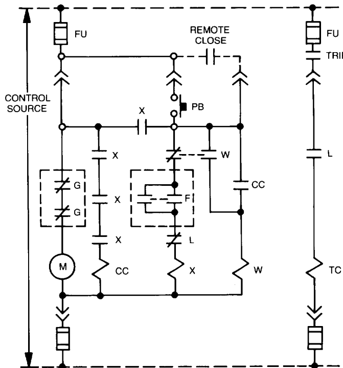
Fig. 5 Elementary diagram for electrically operated drawout breaker. Contact positions are shown with breaker open and closing springs discharged.
