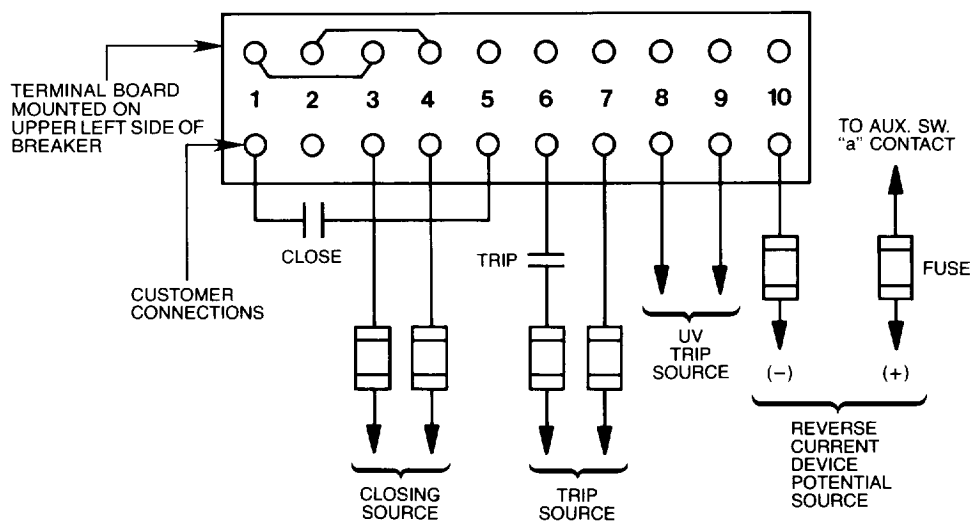
Fig. 3 Control connections to stationary breakers — front view.
