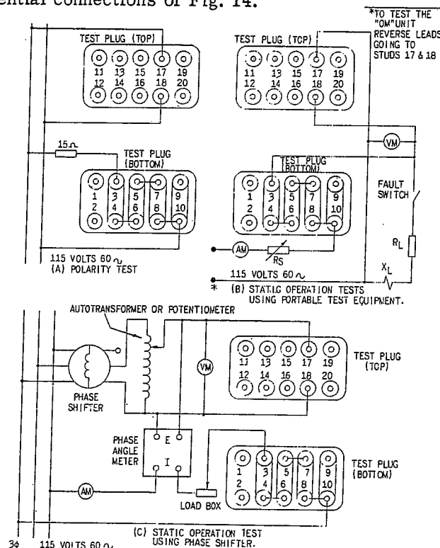
Fig. 13 Test Connections For CEYB12A Relay Using Test Plug (Model XLA12A)
