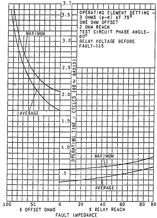
Fig. 9 Operating Characteristics Of The Normally Closed Contacts Of The OM Unit At 10 Amperes Fault Current
