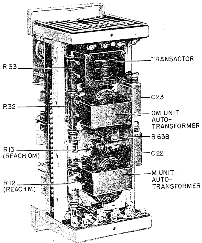
Back View
