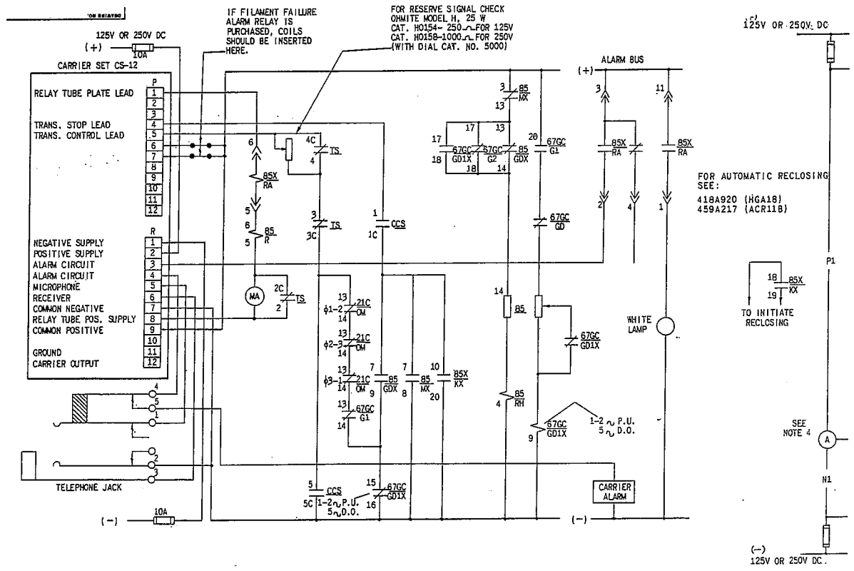
Fig. 14 Elementary Diagram For Carrier Pilot Relaying With Type CEYB12A Relays
