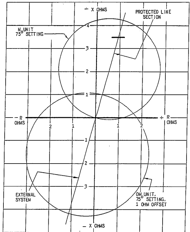
Fig. 10 Typical Static Operating Characteristics Of The Type CEYB12A Relay
