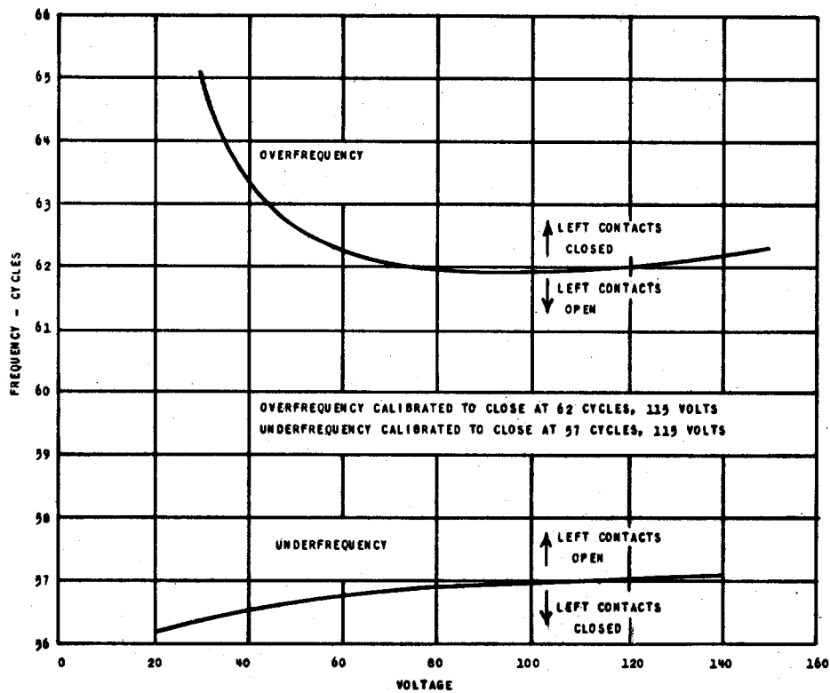
Fig. 2 (K-6556561-0) Voltage-Frequency Curve For Type CFF Relays
