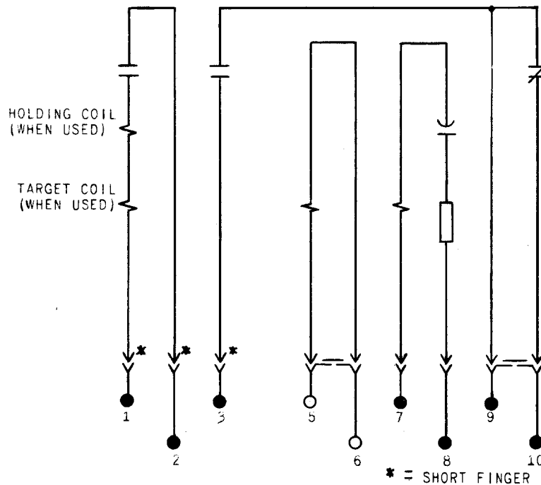
Fig. 1 Internal Connections for the Type CFPP15A Relay (Front View)
