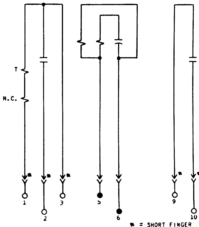
Fig. 1 Internal Connections For Type CFV17A Relay
