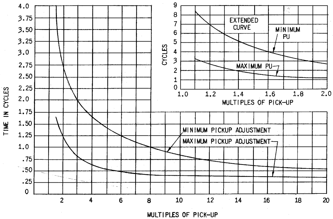
* Fig. 2 Time-Current Characteristics Of The Overcurrent Units Of Type CKPG Relay
