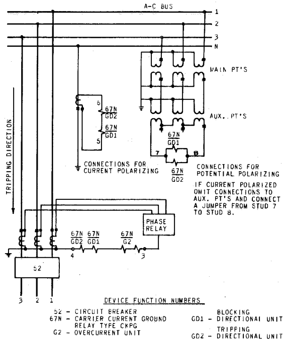
Fig. 9 External Connections for Type CKPG11A Relay
