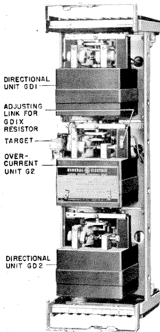
Fig. 5 Type CKPG11A Relay, Unit In Cradle (Front View)
