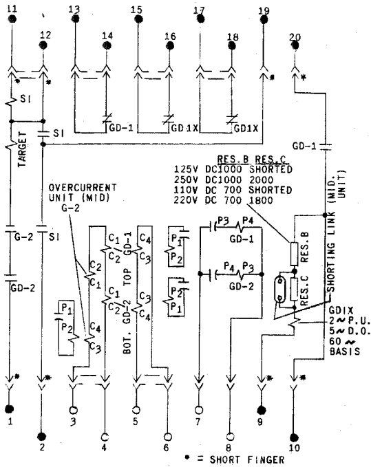
Fig. 8 Internal Connections for Type CKPG11A Relay
