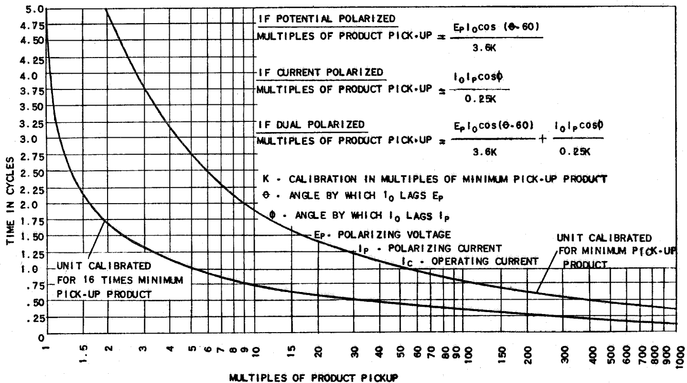
Fig. 3 Time Characteristics Of Dual-Polarized Directional Units GD1 And GD2, Contact Closing Time
