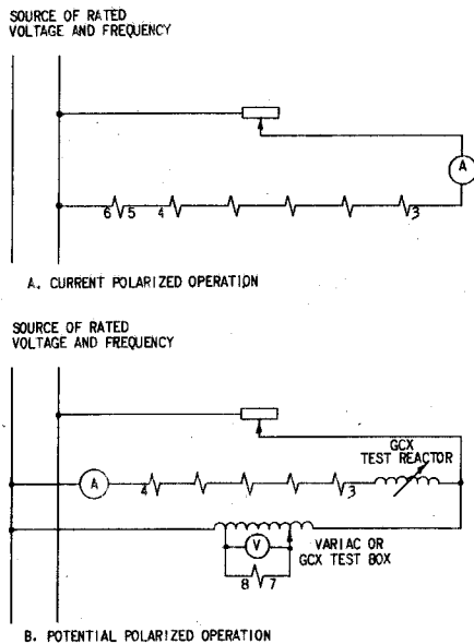
THESE CONNECTIONS PRODUCE TORQUE TENDING TO CLOSE THE NORMALLY OPEN CONTACTS OF ALL UNITS. REVERSING THE CONNECTIONS OF STUDS 5 AND 6 OR 7 AND 8 WILL REVERSE THE TORQUE OF THE GD UNIT ONLY.
