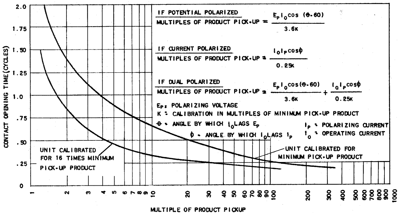
Fig. 4 Time Characteristics Of Dual-Polarized Directional Unit in Type CKPG Relay (Contact Opening Time Of GD1 And GD2 Unit)
