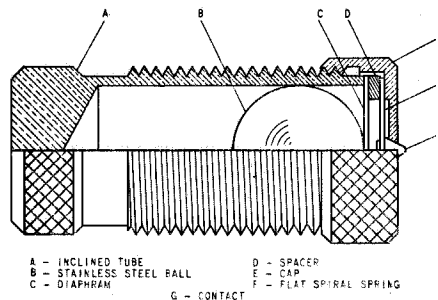
Fig. 7 Stationary Contact Assembly
