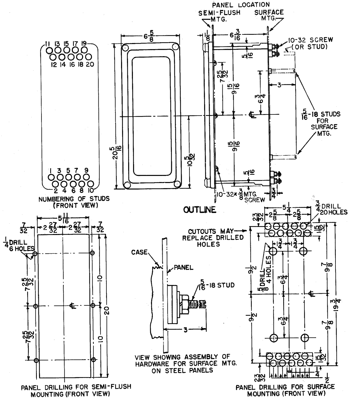
Fig. 11 Outline and Panel Drilling Dimensions for Type CKPG Relay
