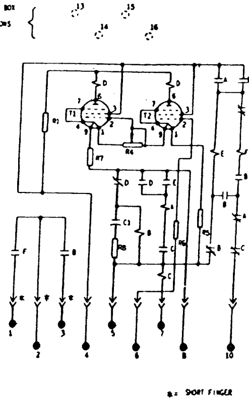
Fig. 6A (0165A7500-1) Internal Connections of Relay Type GES11F (110/125 V.D.C.) Forms 21 and Up (Front View)
