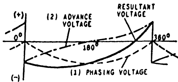
Fig. 3A (K-6400799-1) Components Of Voltage That Control D When Bus And Machine Voltages Are Balanced
