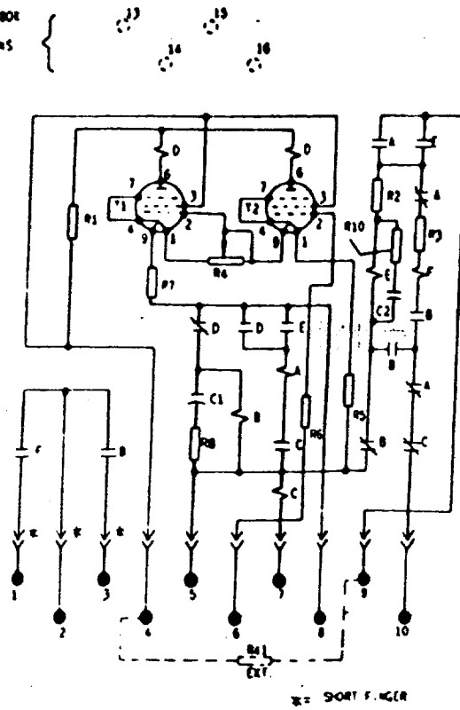
Fig. 6 (0165A7501-1) Internal Connections of Relay Type GES11F (220/250 V.D.C.) Forms 21 and Up (Front View)
