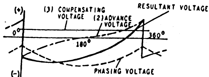
Fig. 3B (K-6400799-1) Components Of Voltage That Control D When Bus And Machine Voltages Balance
