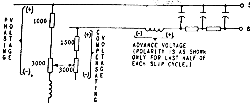
Fig. 3C (K-6400799-1) Elementary Diagram - Components Of Voltage That Controls D Relay
