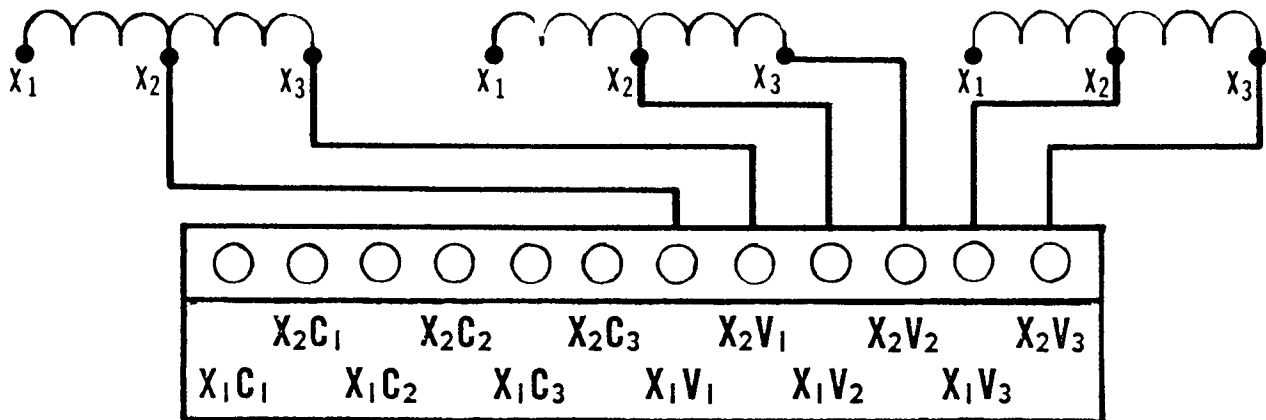
Fig. 2. Connections for high ratio
