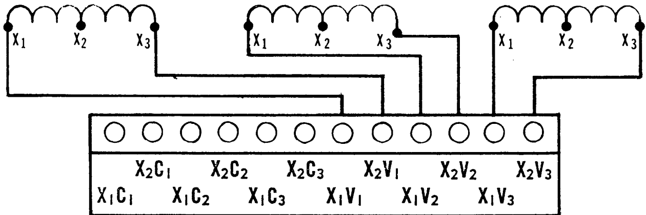
Fig. 1. Connections for low ratio
