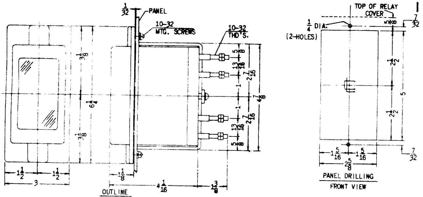
Fig. 6 Outline and Panel Drilling Diagram for HGA148B Relay (Semi-flush Mounted)
