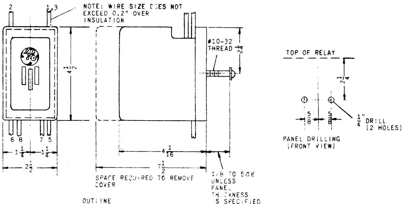
Fig. 3 Outline of External Resistor Used With HGA14BA and HGA14BB Relays
