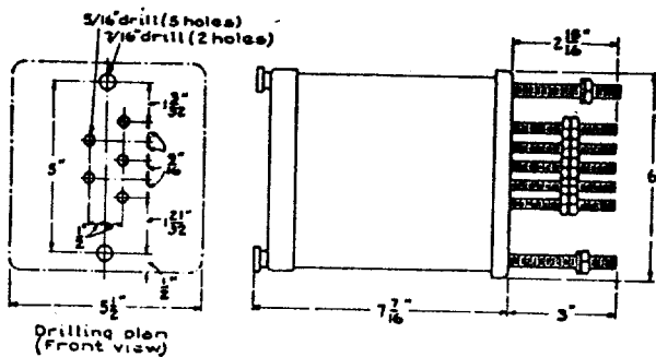
Fig. 20. Dimensions of IAC12A Relay (Also IAC12C)
