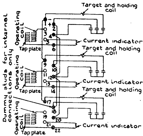
Fig. 14. Internal Connections of IAC12D Relay
