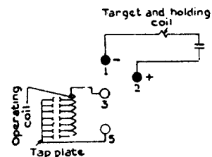
Fig. 4. Internal Connections (Back View)
