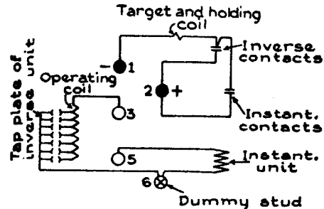
Fig. 17. IAC11E Internal Connections
