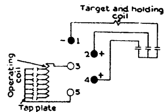
Fig. 21. Internal Connections of IAC12A Relay
