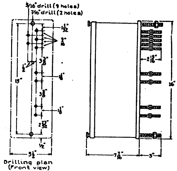
Fig. 23. Dimensions of IAC12B Relay
