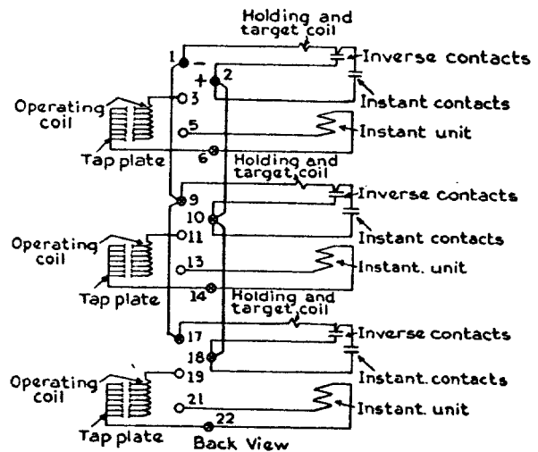
Fig. 18. IAC11H Internal Connections
