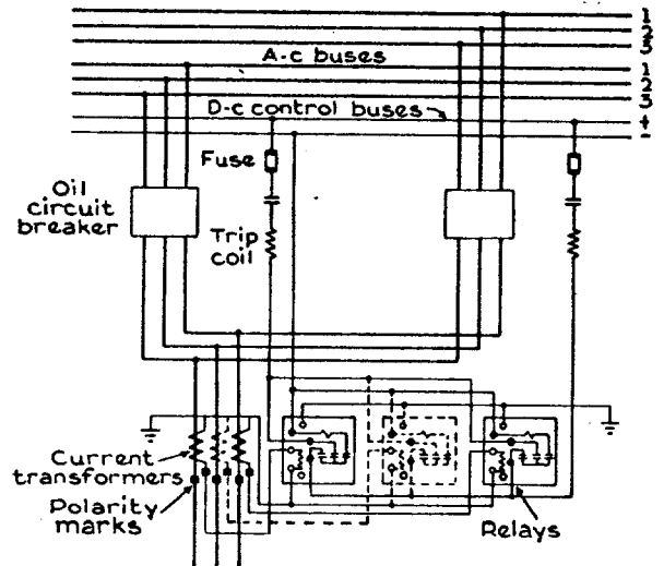
Fig. 15. Wiring Diagram Showing External Connections of IAC12C Relay
