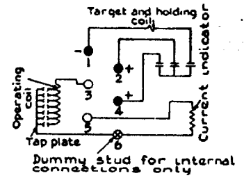
Fig. 13. Internal Connections of IAC12C Relay
