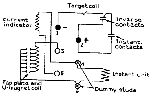
Fig. 16. IAC11F Internal Connections
