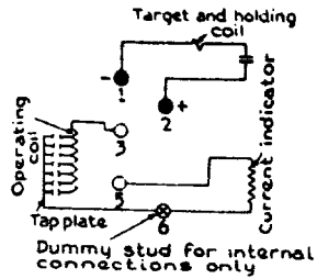
Fig. 11. Internal Connections of IAC11C Relay
