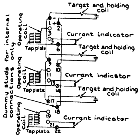
Fig. 12. Internal Connections of IAC11D Relay
