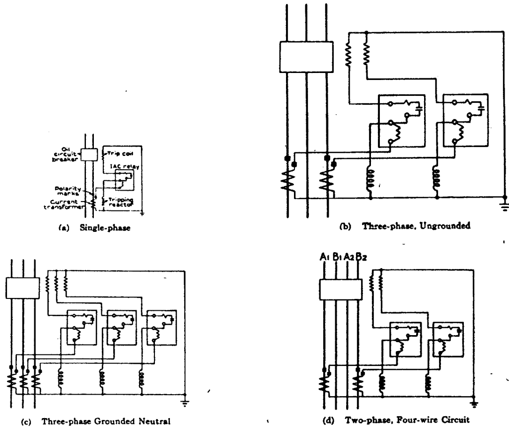
Fig. 6. Typical Wiring Diagrams, Using Relays with Tripping Reactors
