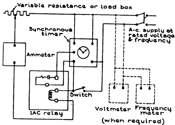
Fig. 8. Connections for Testing Single-phase Relay
