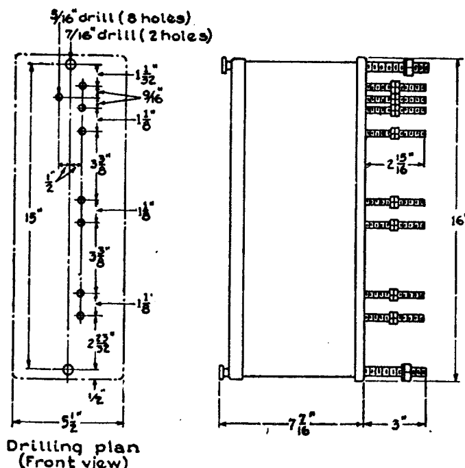
Fig. 9. Dimensions of IAC11B Relay (Also IAC11D and IAC11E)
