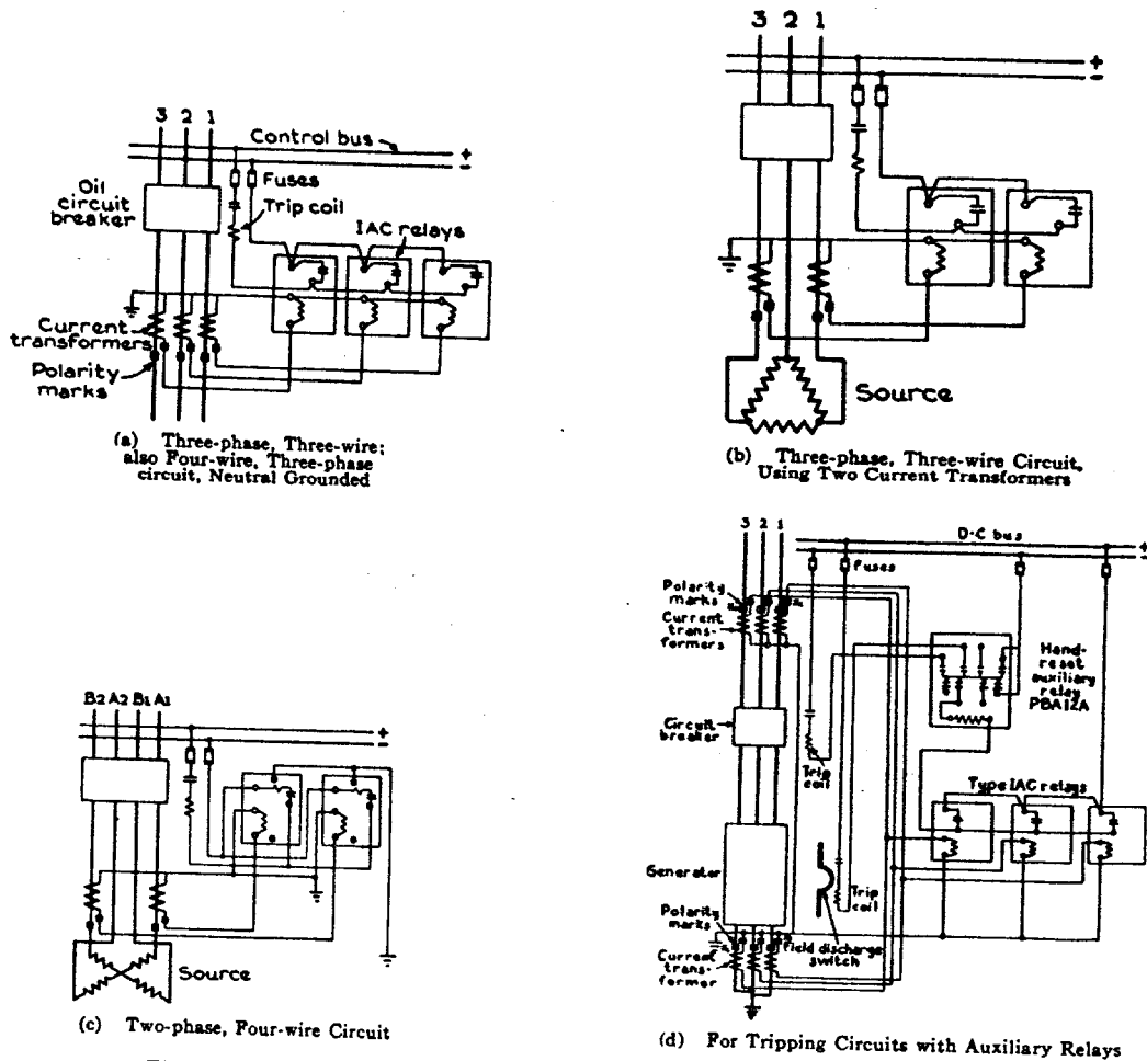
Fig. 5. Typical Wiring Diagrams, Using Relays with D-c Control Power
