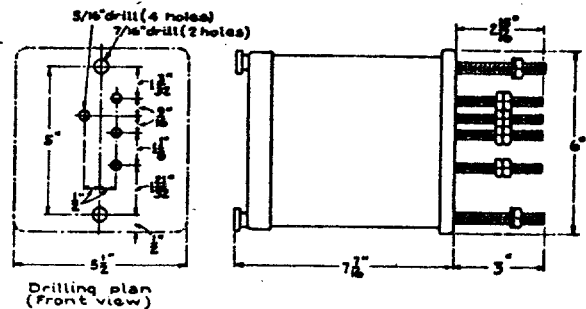
Fig. 3. Outline Dimensions and Panel Drilling
