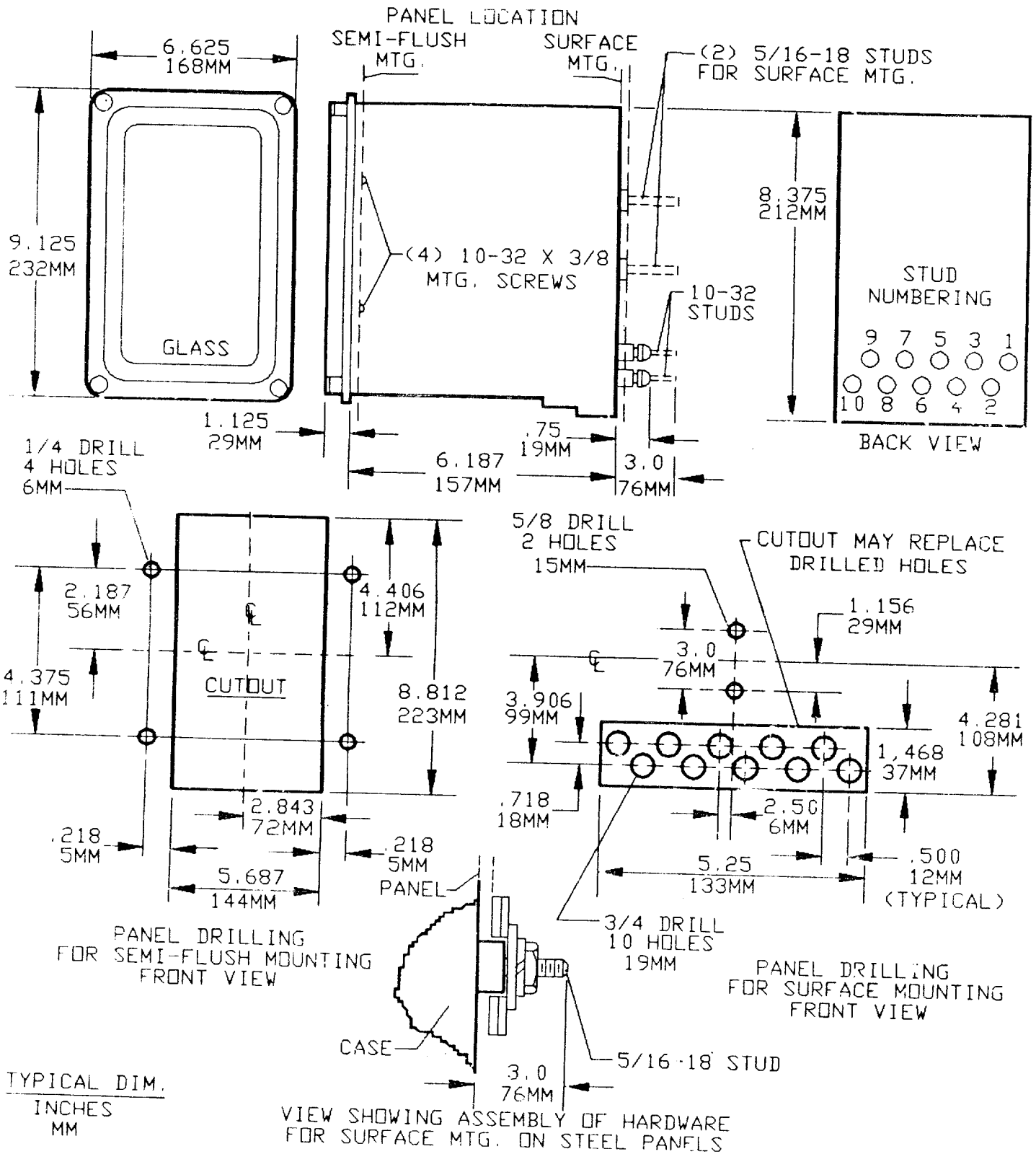
*Fig. 12 (K-6209271 [8]) Outline and Panel Drilling Dimensions for Type IJF Relays
