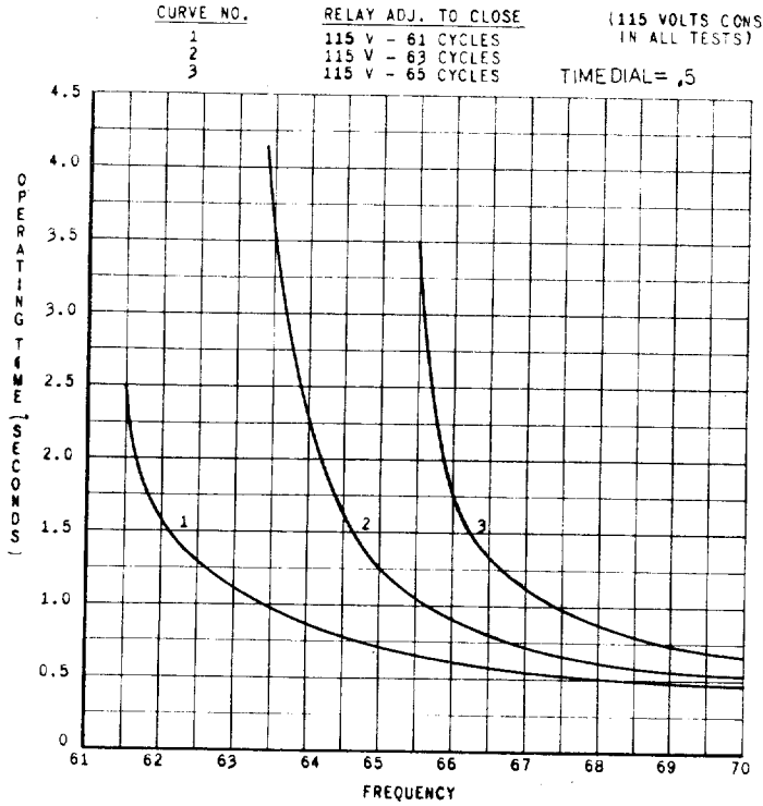
Fig. 4 Type IJF51A Relay, Time-Frequency Characteristics
