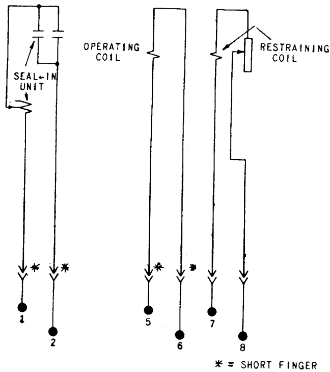
*Fig. 7 (K-6306813 [2]) Type IJF51A Relay, Internal Connections (Front View)
