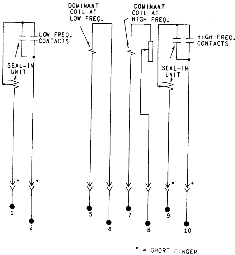
*Fig. 9 (K-6400202 [2]) Type IJF52A Relay, Internal Connections, (Front View)
