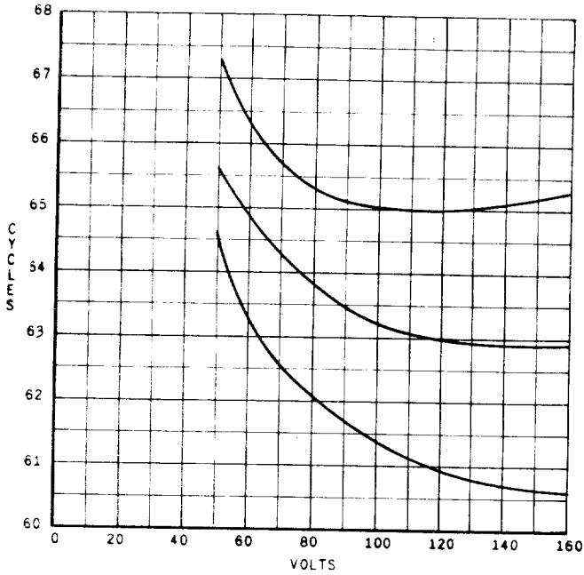
Fig. 3 Type IJF51A Relay, Voltage-Frequency Characteristics
