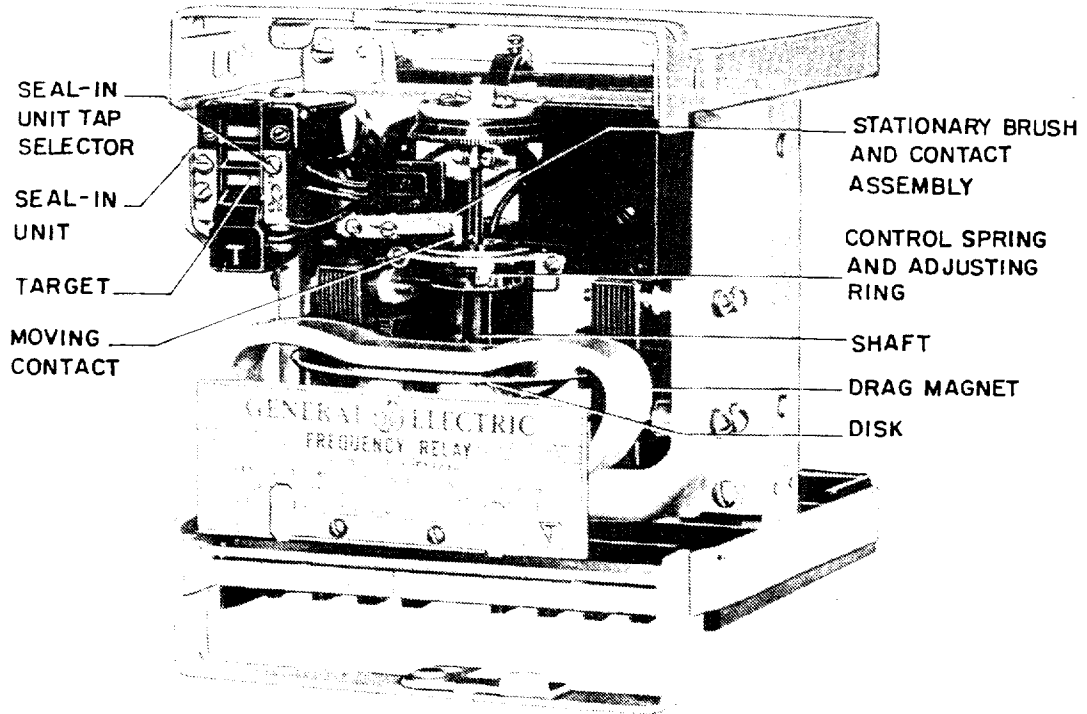
Fig. 1 Type IJF Relay Removed From Case (Front View)
