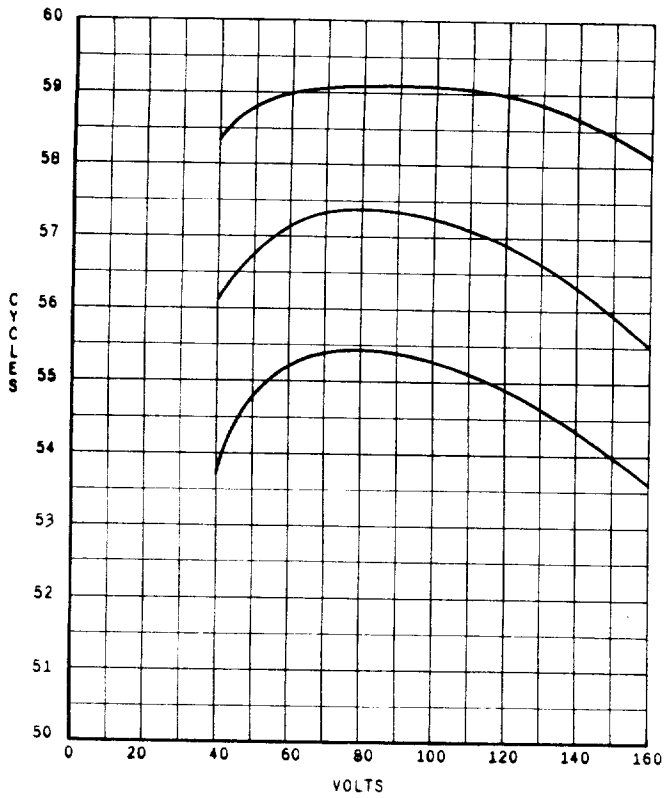
Fig. 5 Type IJF51B Relay, Voltage-Frequency Characteristics
