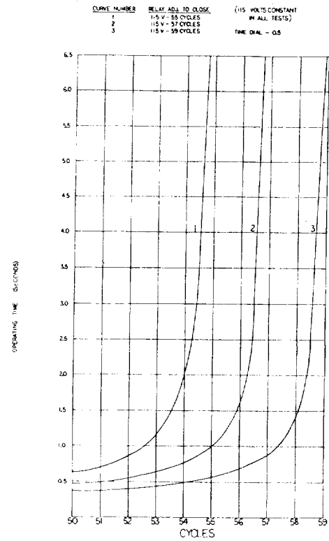
Fig. 6 Type IJF51B Relay, Time-Frequency Characteristics
