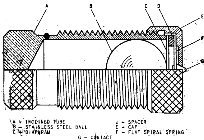
FIG. 2 (418A859-0 SH. 2) Internal Connections For Type JBC53L Relay
