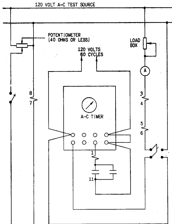
FIG. 6 (418A973-0) Test Connections For Checking Pickup And Operating Time Of The Time Overcurrent Unit
