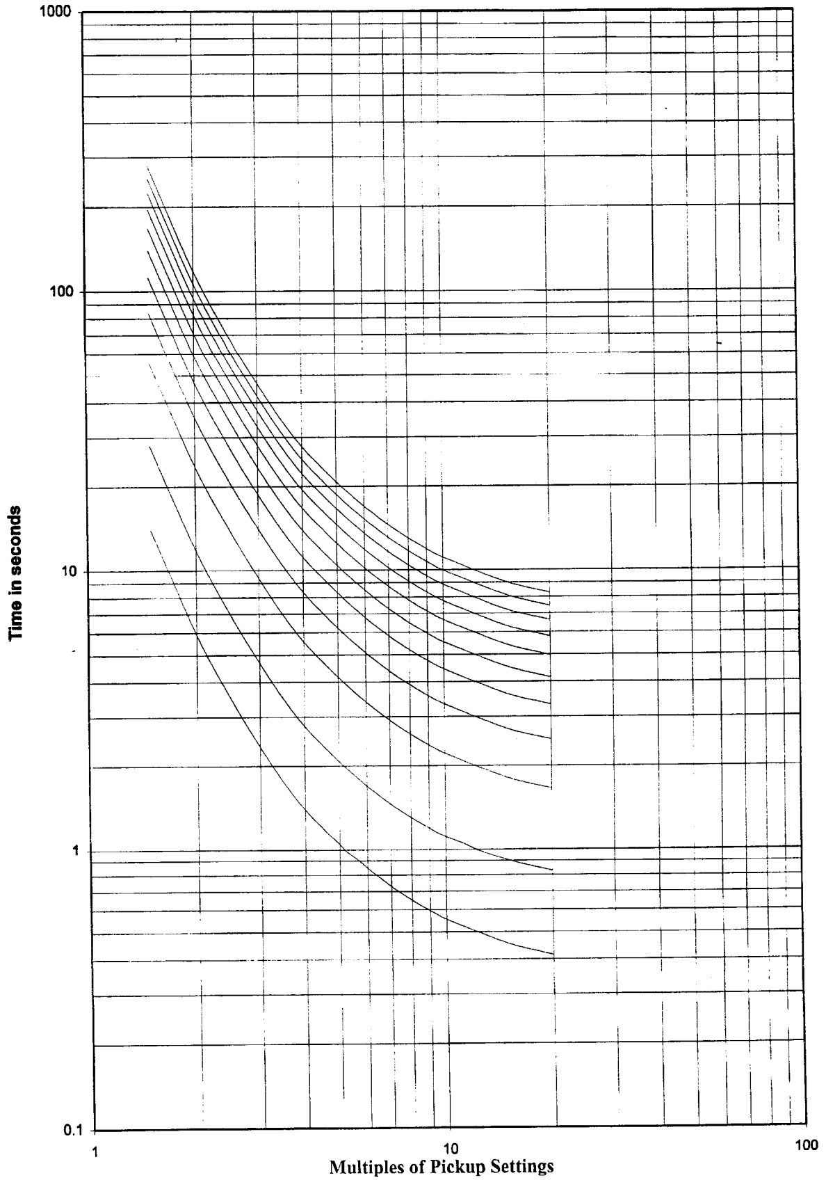
Figure 2 (0385A1101) Long Time Very Inverse Curve
