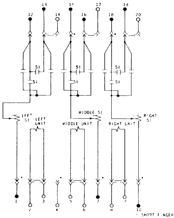
Figure 5 (6375726-5) Internal Connections Diagram for the PJC32C Relay (Front View)
