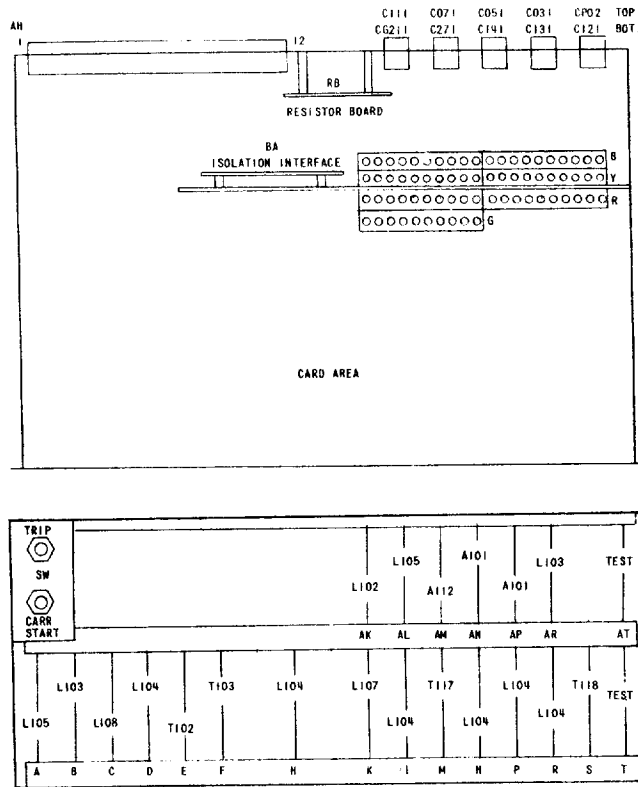
FIG. 3 (0246A6850-0) Component Locations For The Type SLA51A Relay
