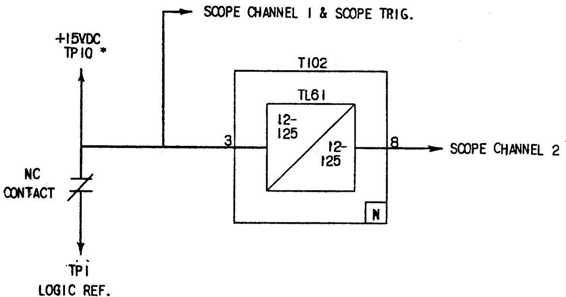
FIG. 6 (0208A5504AJ-1) Isolation Interface Circuit
