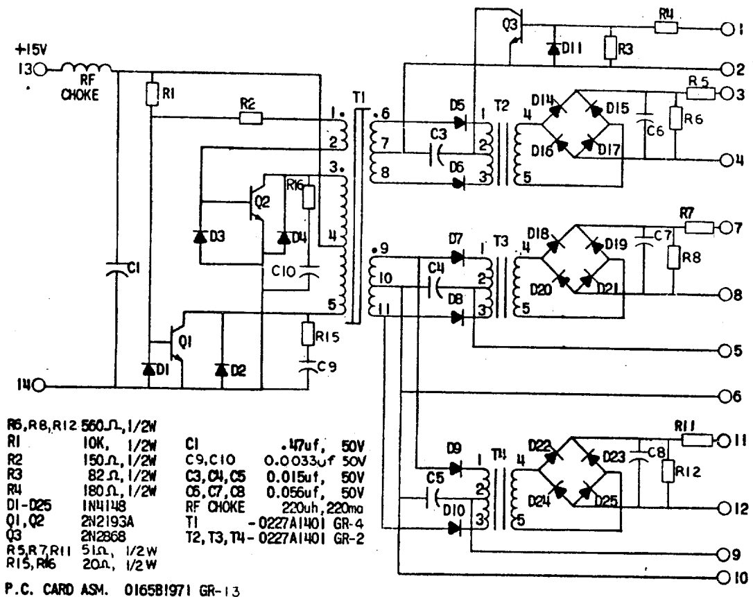
FIG. 6 (0208A5504AJ-1) Isolation Interface Circuit
