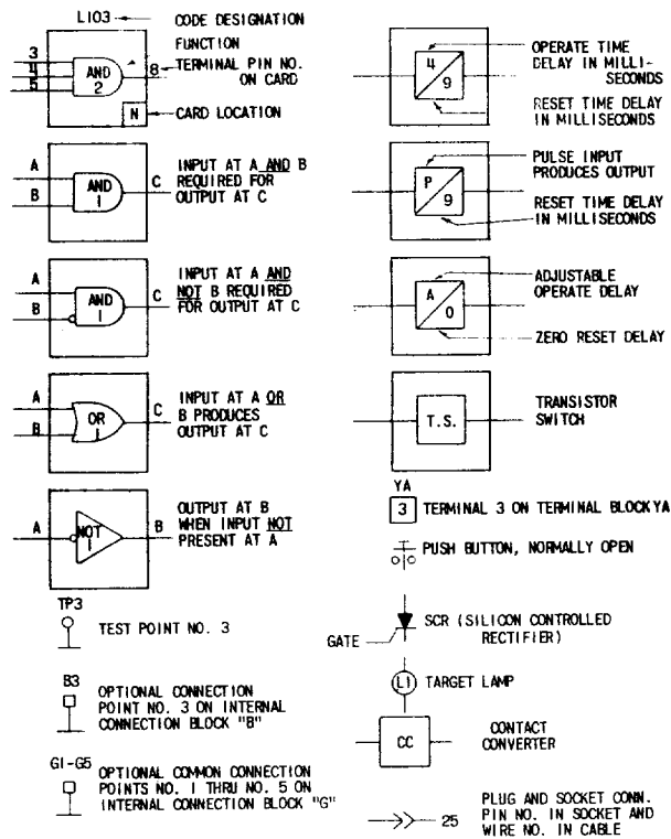
FIG. 4 (0227A2047-0) Logic And Internal Connection Diagram Legend
