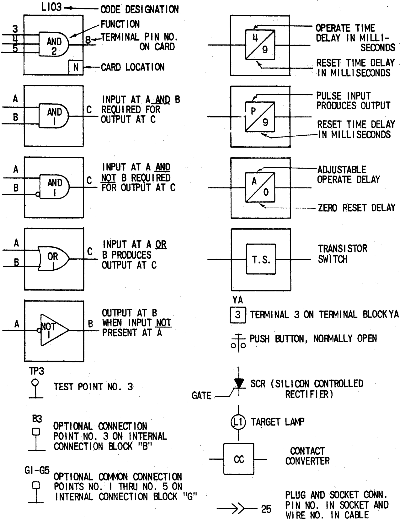
FIG. 4 (0257A2047-0) LOGIC AND INTERNAL CONNECTION DIAGRAM LEGEND
