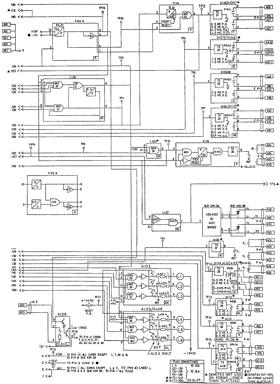
Figure 2B (0172C5115-13) Internal Connections Diagram for the Type SLAT51J (Forms 11 and up)
