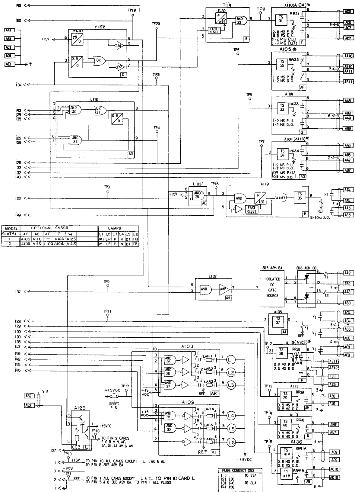
Figure 2A (0171C7886-3) Internal Connections Diagram for the Type SLAT51J (Forms 1 and 2)
