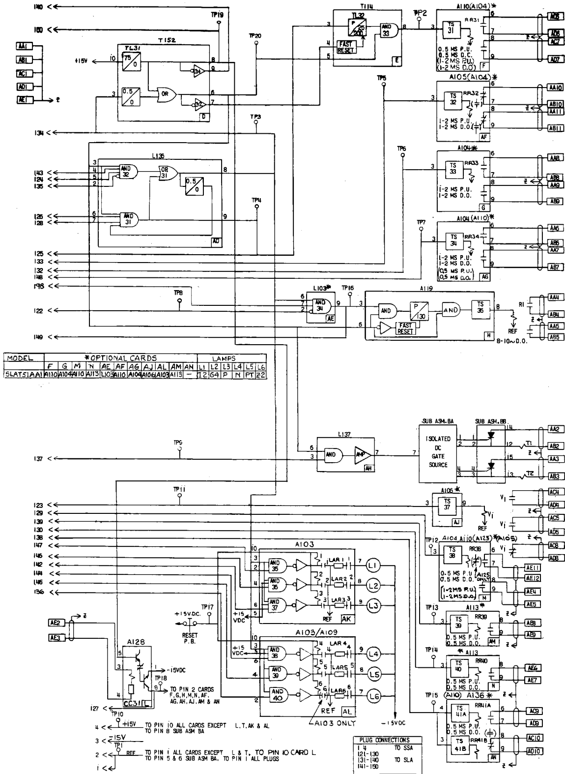
Fig. 2 (0179C6174-0) Internal Connections Diagram for the Type SLAT51AA Relay
