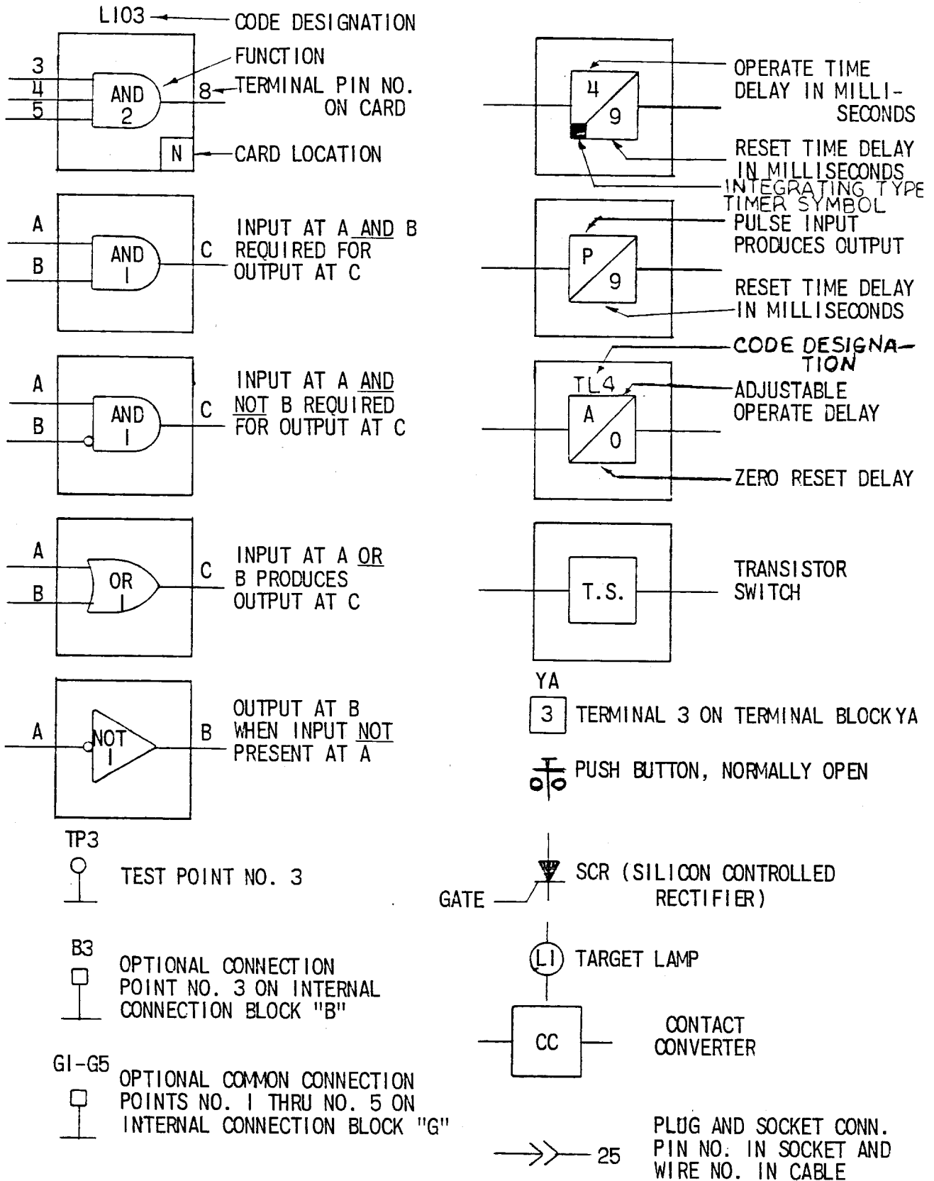
Fig. 3 (0227A2047-1) Internal Connection Diagram Legend
