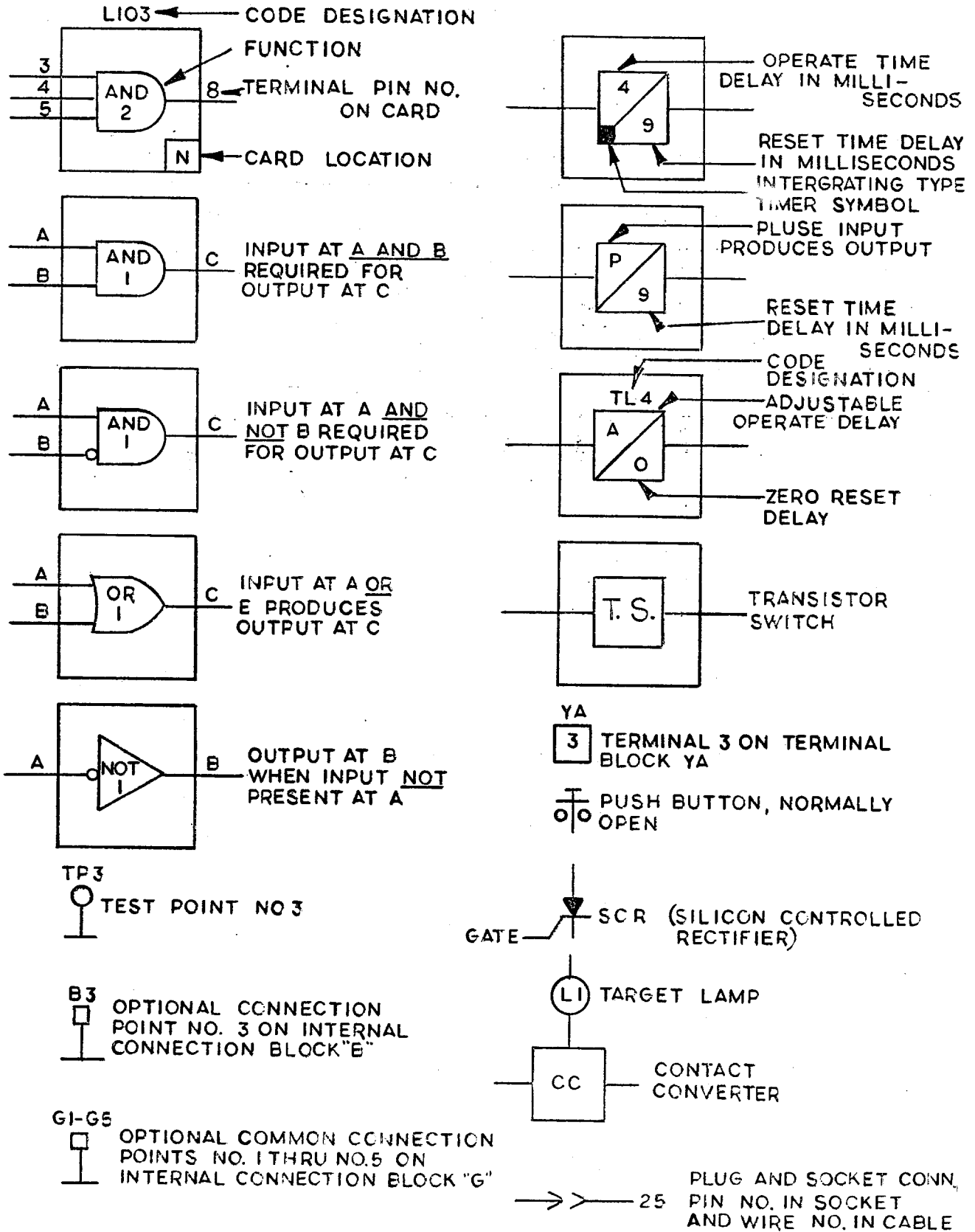
Figure 2 (0227A2047-1) Logic Legend for Internal Connection Diagram
