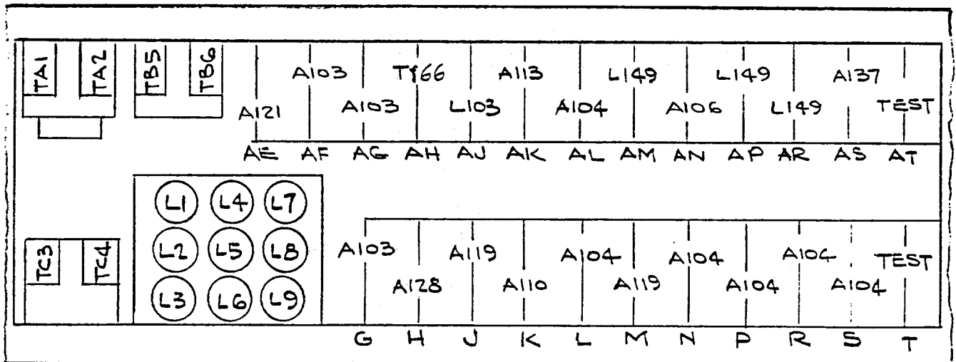
Figure 5 (0285A7045-0) Component Location Diagram for the SLAT53L Relay
