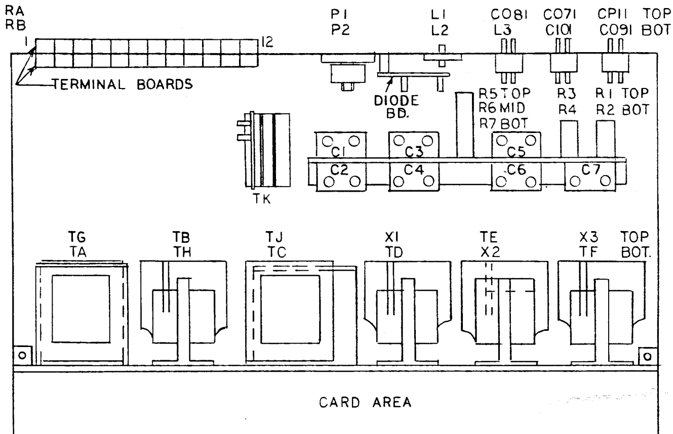
PLAN VIEW (COVER REMOVED)
