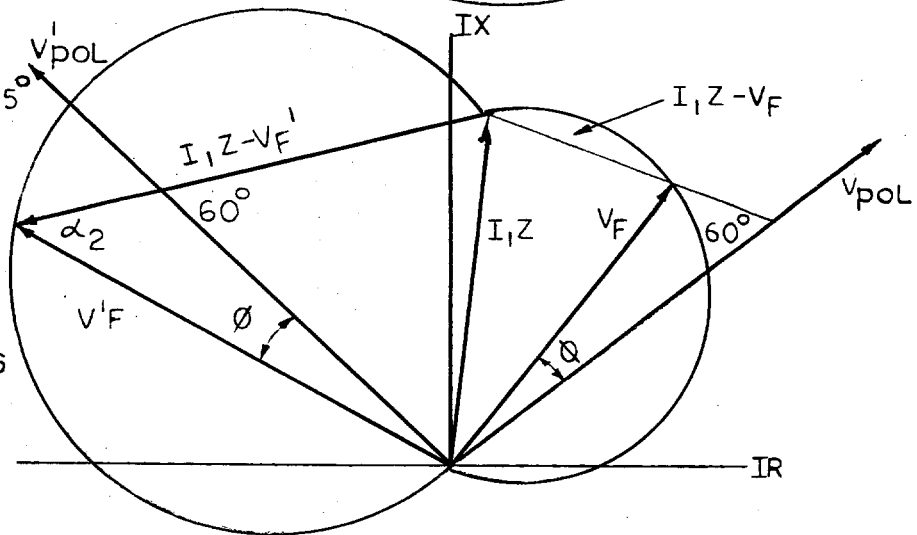
Figure 11 (0246A6866-0) Effect of Polarizing Phase Shift on an Mho Characteristic
