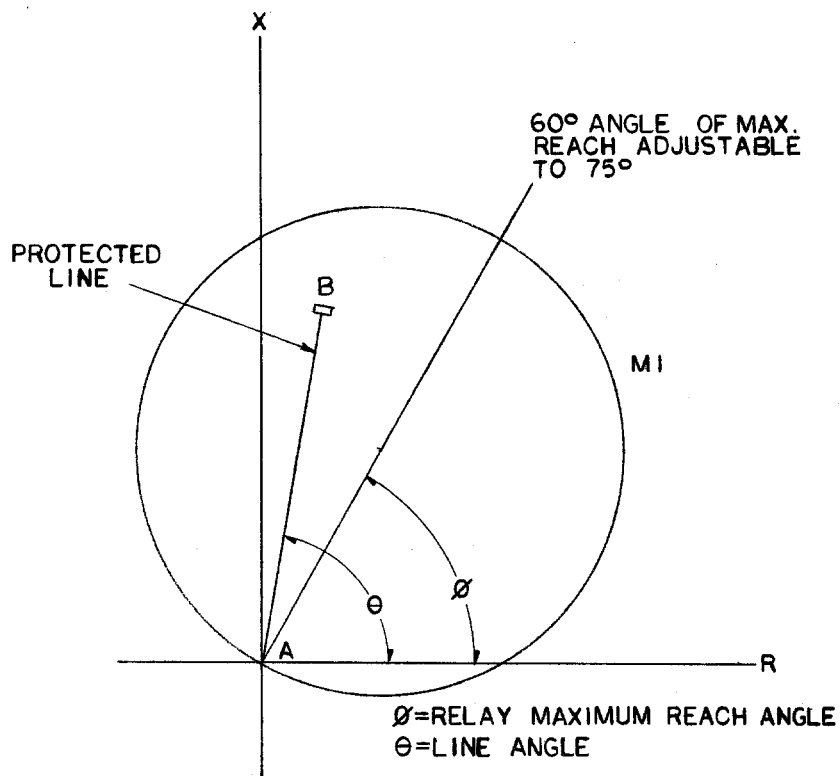
FIG. 5 (0269A1709-0) Typical MI Characteristic for the Type SLY52A Relay.
