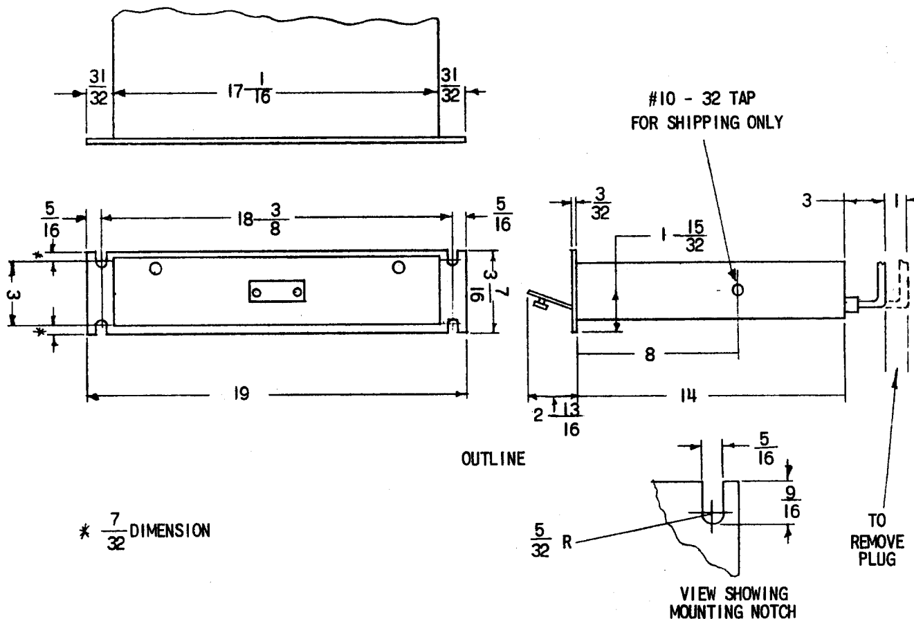
FIG. 1 (9227A2036-0) Outline and Mounting Dimensions for the Type SLY52A Relay.
