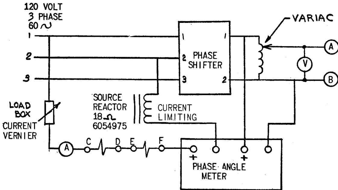
FIG. 14 (0178A7029-3) Phase Shifter Test Circuit
