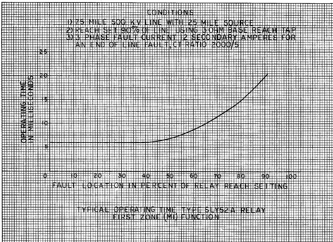
FIG. 4 (0257A8491-0) Typical Operating Time for the Type SLY52A Relay
