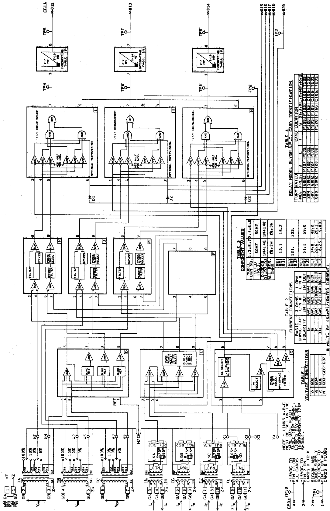
Fig. 2 (0136D5011-0) Internal Connections Diagram for the SLYG61A Relay
