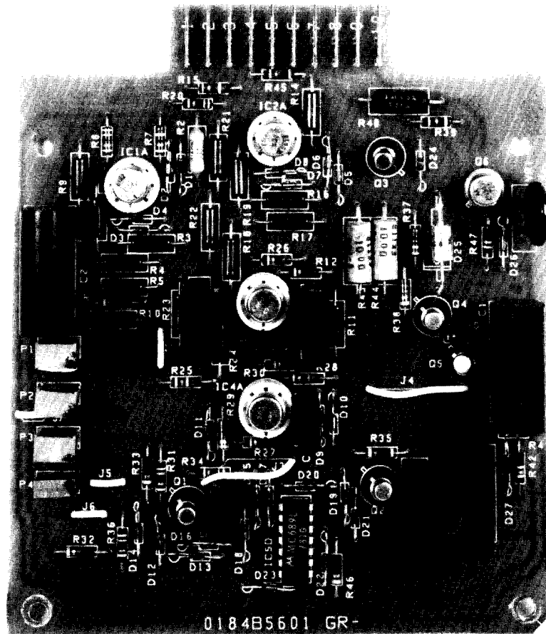
Figure 24 (8043291) Printed-Circuit Card
