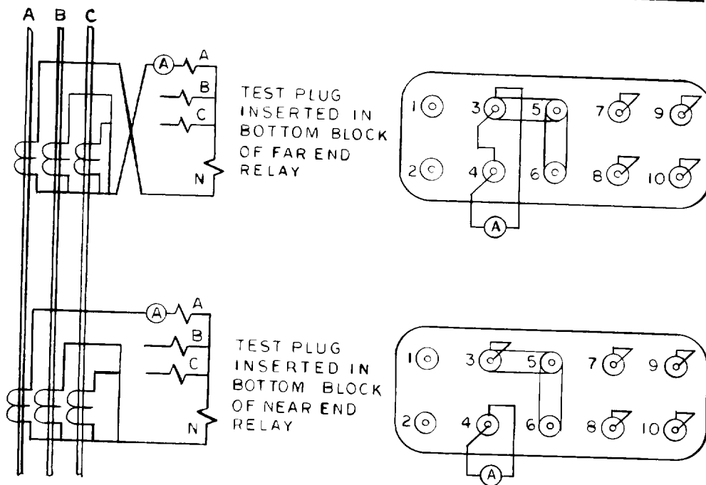
Figure 17 (0275A2021) Test Connections Diagram for Test 6
