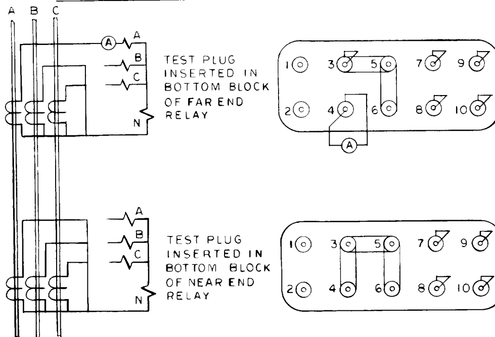
Figure 15 (0275A2019) Test Connections Diagram for Test 4
