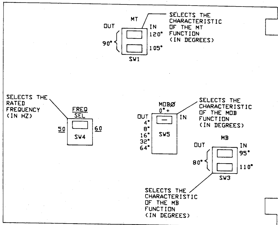
Figure MO-15 (0285A9977) Internal Switches, UTM112 Module
