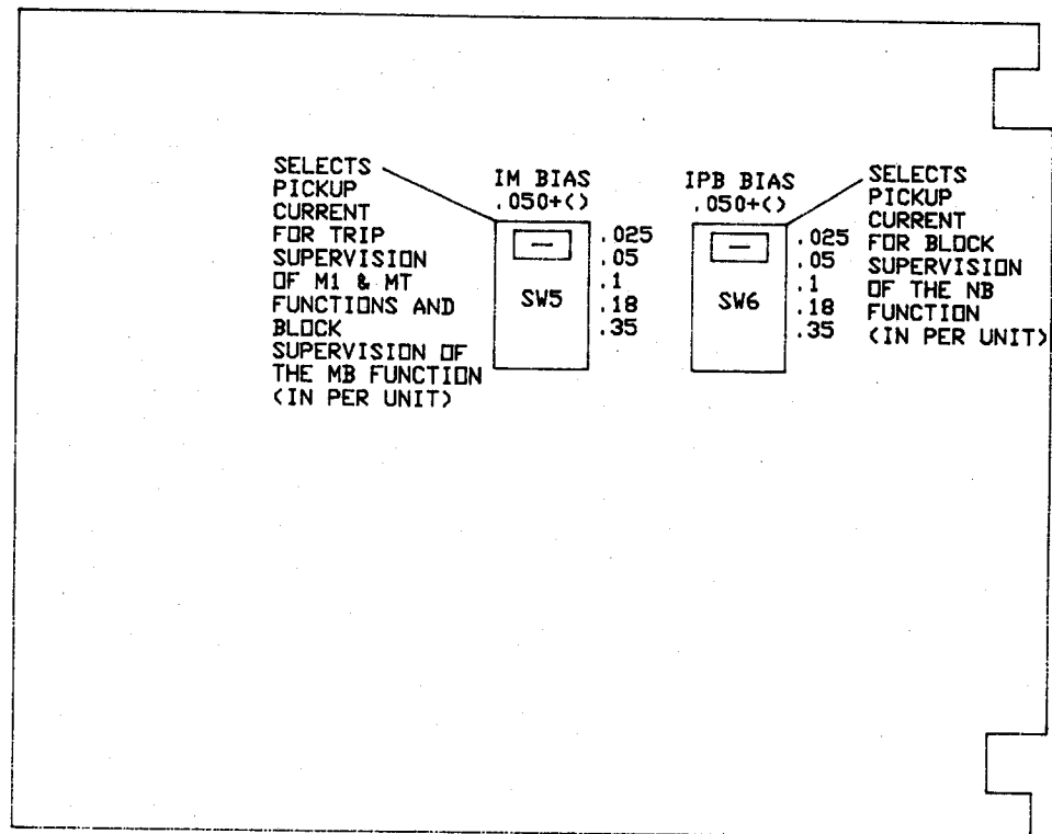
* Figure MO-3 (0286A2829 [1]) Internal Switches, ADM112 Module
