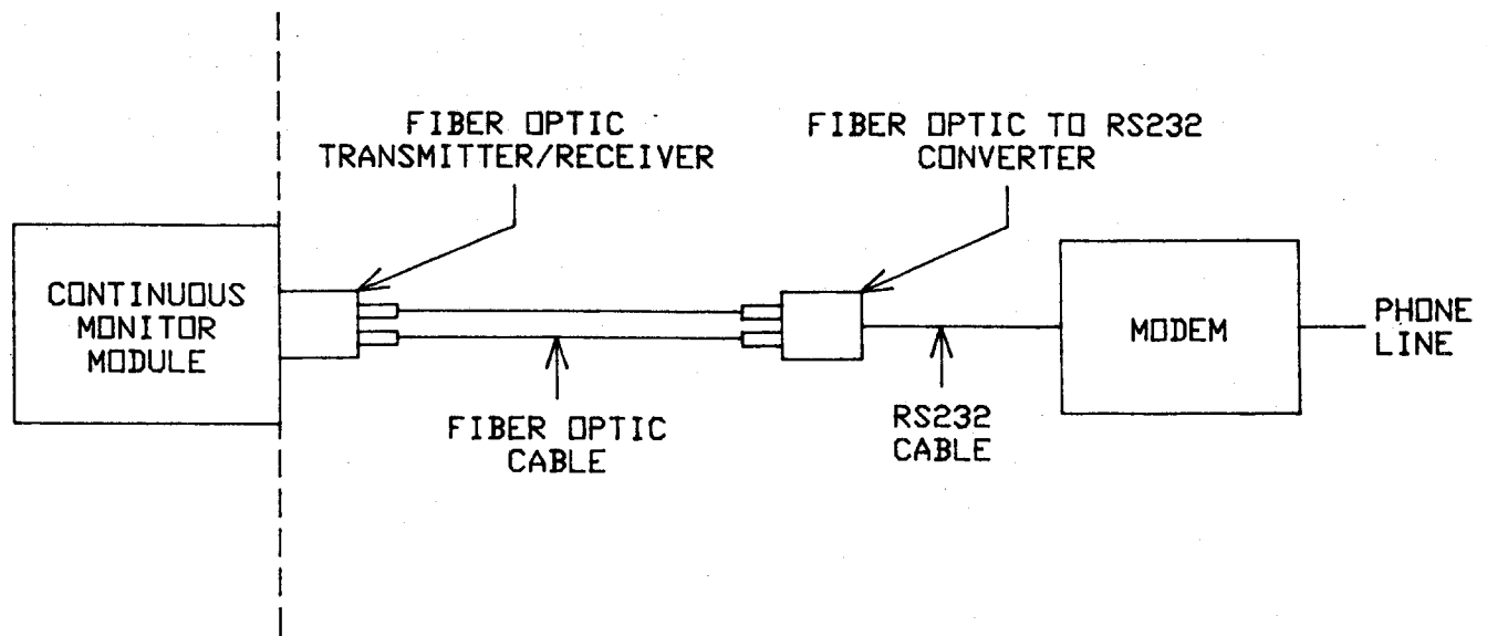
Figure CM-3 (0285A9899-2) Serial Data Link Connection
