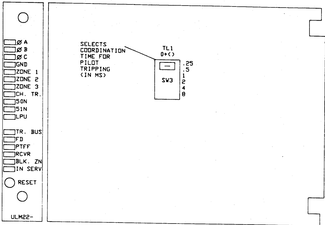
Figure MO-14 (0285A9976) Front Panel & Internal Switch, ULM222 Module
