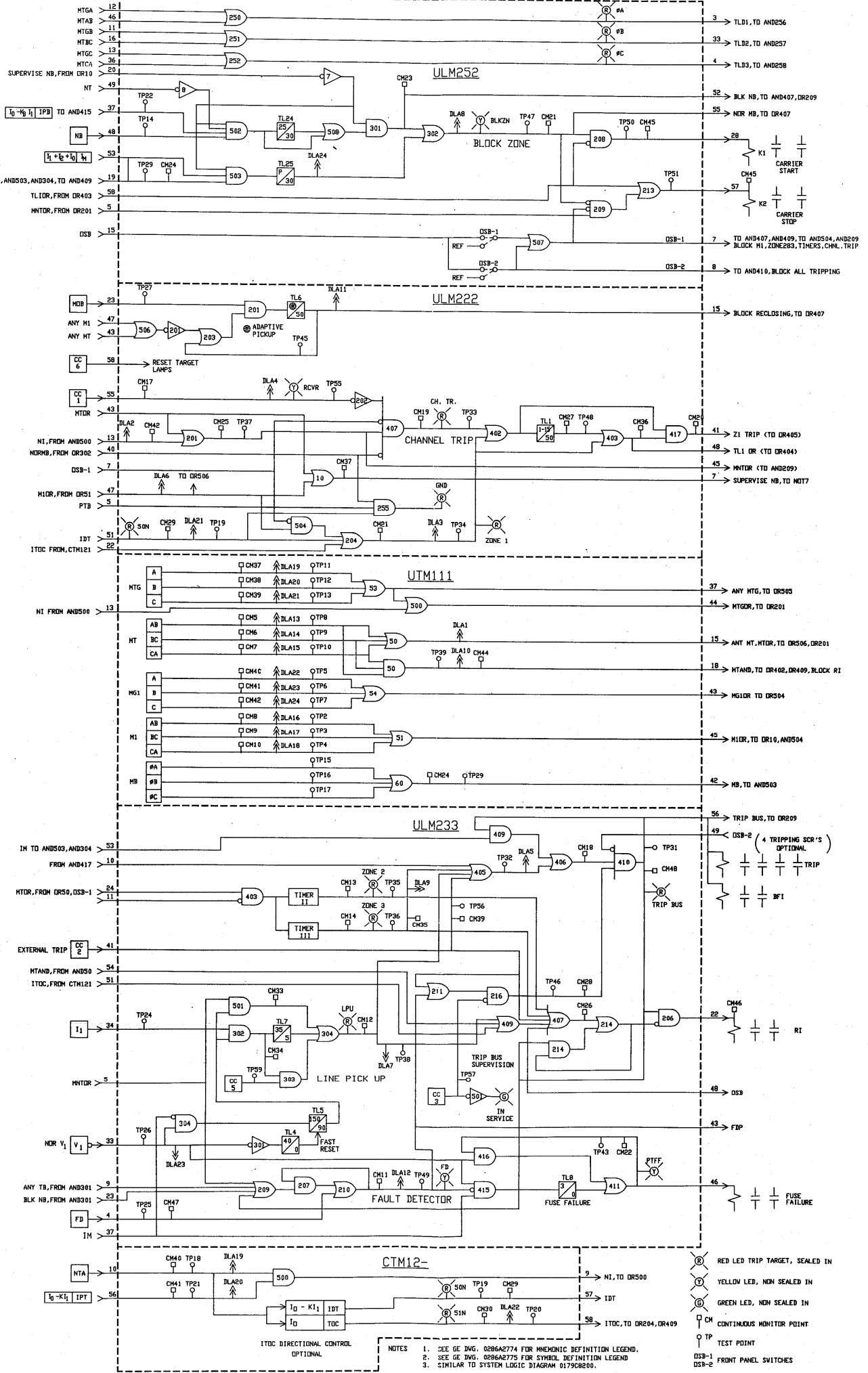
* Figure SE-2 (0153D7643 [3]) Service Logic
