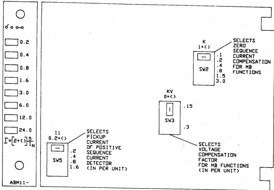
Figure MO-2 (0285A9972) Front Panel & Internal Switches, ABM11(-) Module
