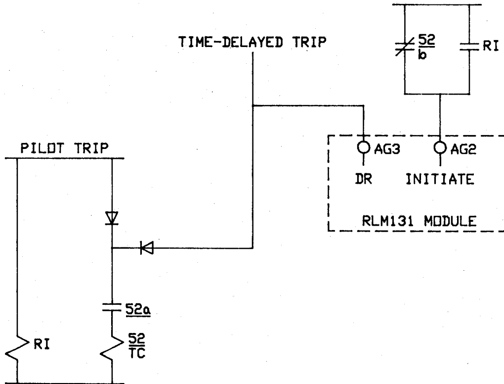
Figure RE-3 (0285A9672-1) Use of BI Contact to Block Instantaneous Trip Prior to First Reclosure
