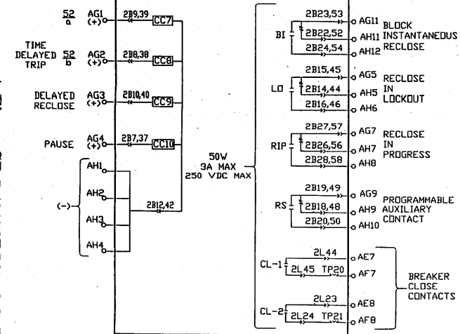
* Figure SD-5 (0163D7654 [1]) Elementary Diagram
