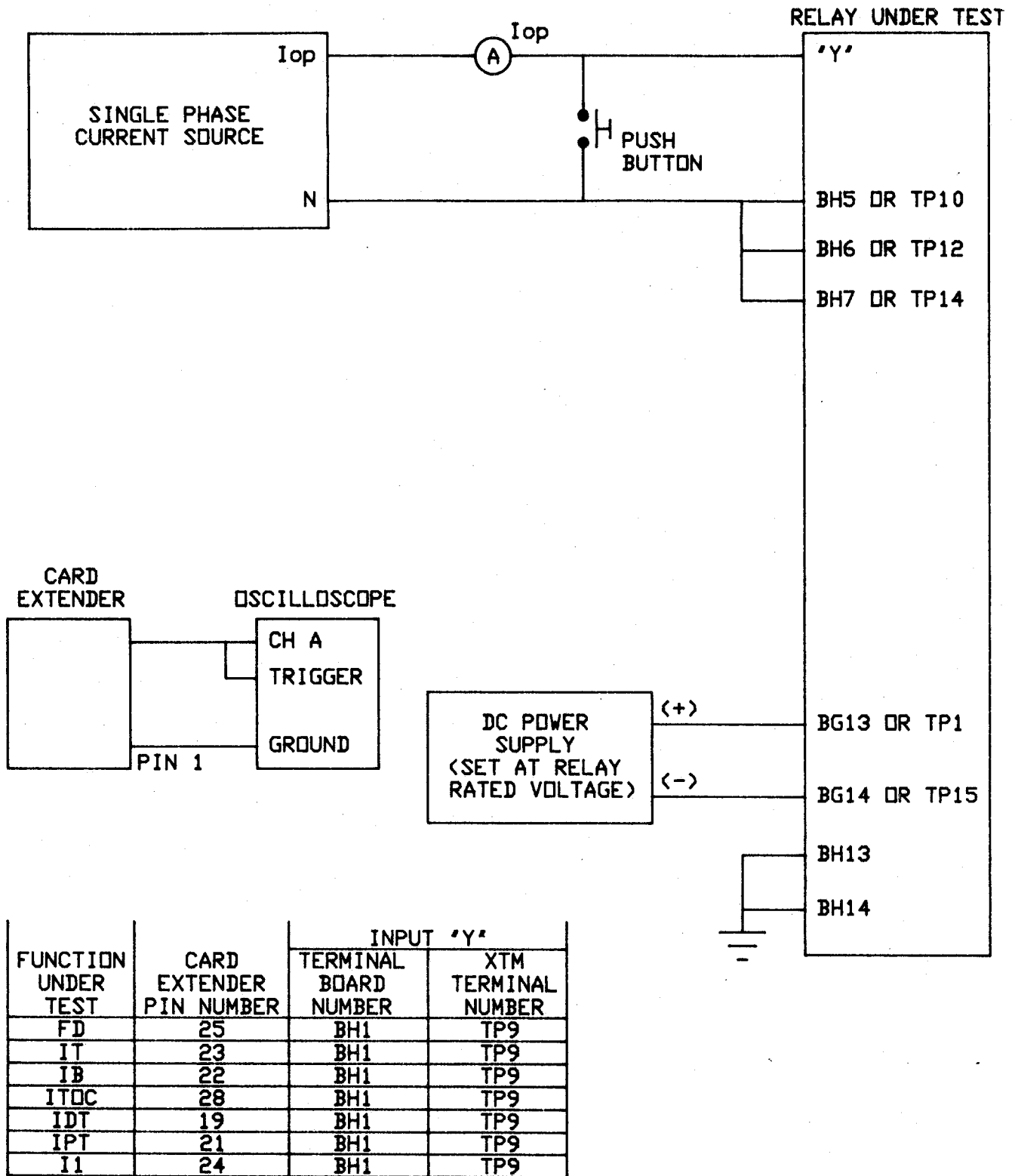
Figure AT-1 (0286A2813) Level-Detector Test Connections
