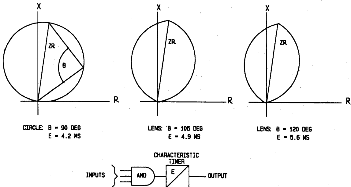
Figure CS-1 (0285A9991-1) Phase Distance Functions Characteristic Shapes
