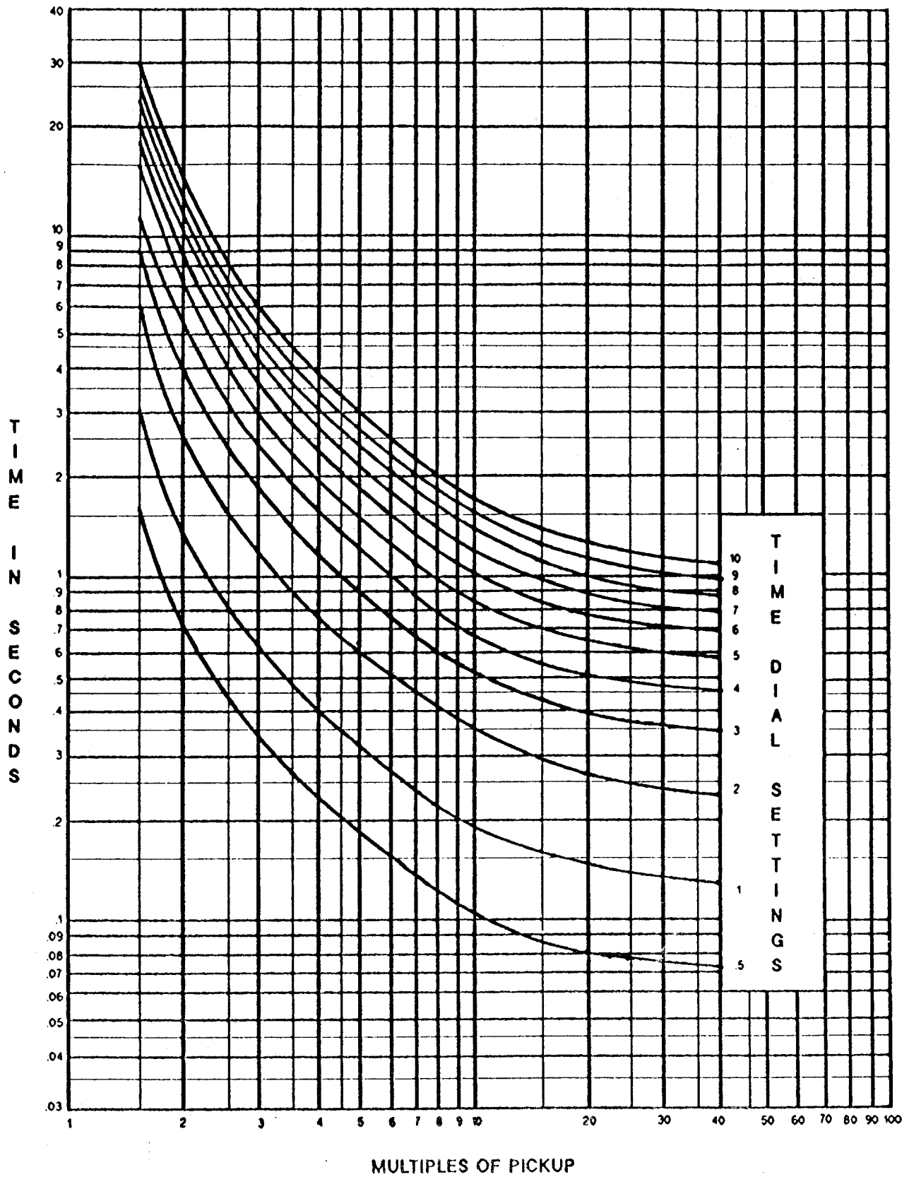
* Figure CS-4 (0285A9858 [1]) Time Curve Characteristics
