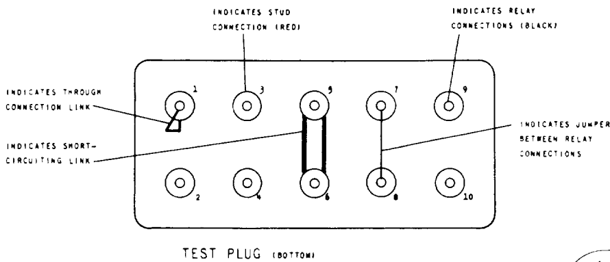
TEST PLUG (BOTTOM)
