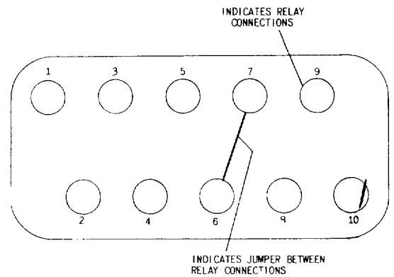
Fig. 10 Conventional Representation of XLA13A Test Plug Connections
