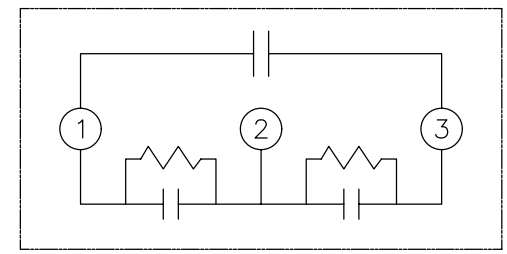
SCHEMATIC DIAGRAM - 304
