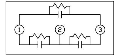
SCHEMATIC DIAGRAM - 302
