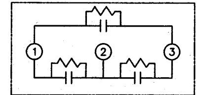
SCHEMATIC DIAGRAM - 302
