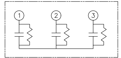
SCHEMATIC DIAGRAM - 337
