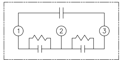
SCHEMATIC DIAGRAM - 304
