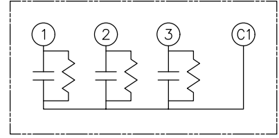
SCHEMATIC DIAGRAM - 322
