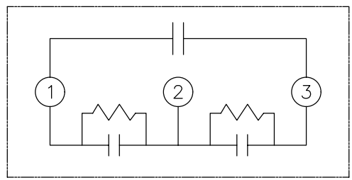
SCHEMATIC DIAGRAM - 304
