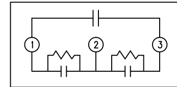
SCHEMATIC DIAGRAM - 304
