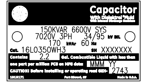
101N171 Rating Plate
