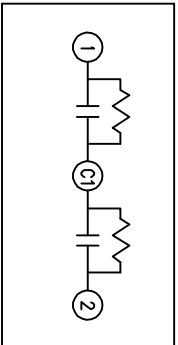
SCHEMATIC DIAGRAM - 227
