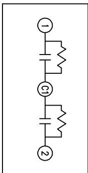
SCHEMATIC DIAGRAM - 227
