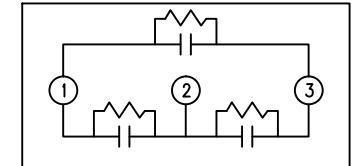
SCHEMATIC DIAGRAM - 302
