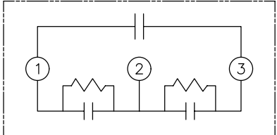
SCHEMATIC DIAGRAM - 304
