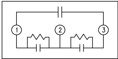
SCHEMATIC DIAGRAM - 304
