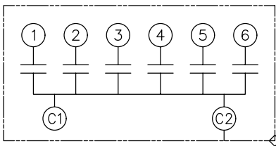
SCHEMATIC DIAGRAM - 601
