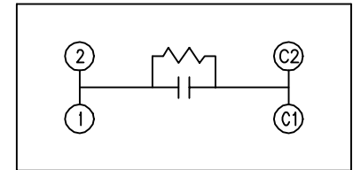
SCHEMATIC DIAGRAM - 107
