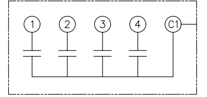
SCHEMATIC DIAGRAM - 401 ◊
