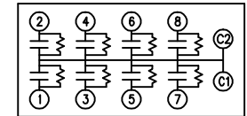
SCHEMATIC DIAGRAM - 802
