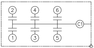
SCHEMATIC DIAGRAM - 606
